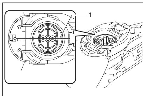
► 1. Alignment line
