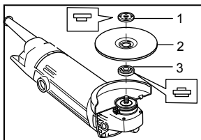
1. Lock nut 2. Depressed center wheel 3. Inner flange
